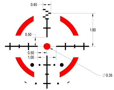
DETAIL D
