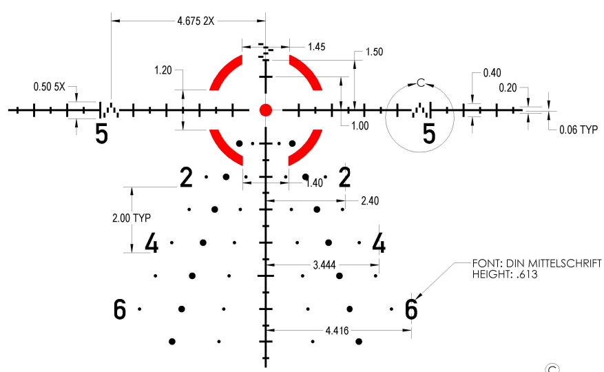
DETAIL B
